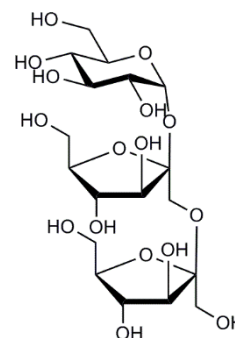
(O-β-D-fructofuranosyl-(2-1)-β-D fructofuranosyl-(2-1)-α-D-glucopyranoside)
